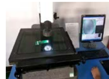
Leather abrasion test
